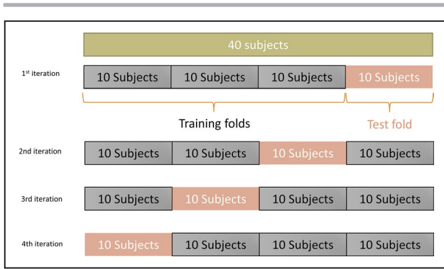
Figure 6. Performance evaluation using 4-fold cross-validation procedure.
